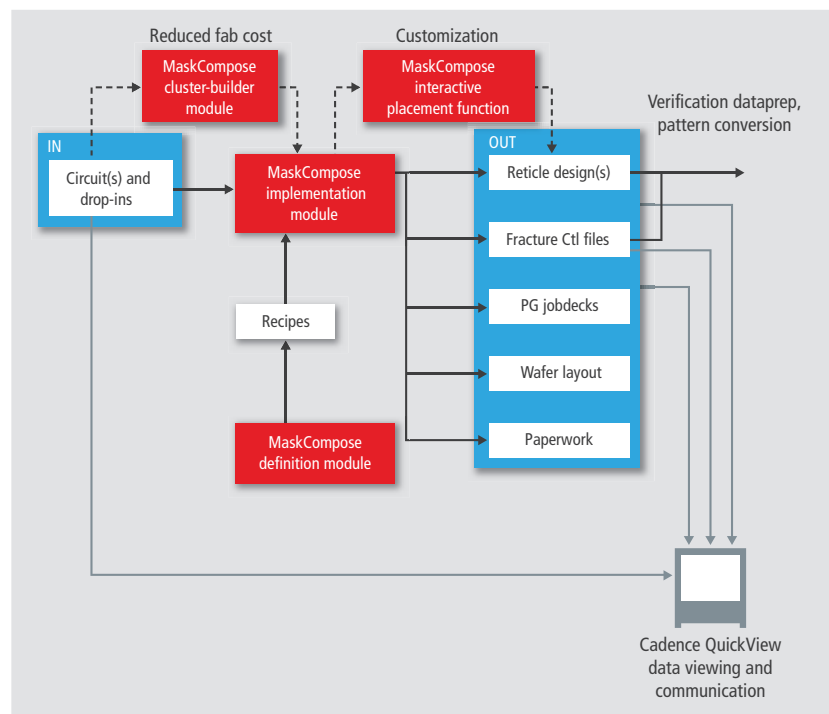
Figure 1: MaskCompose schematic overview
